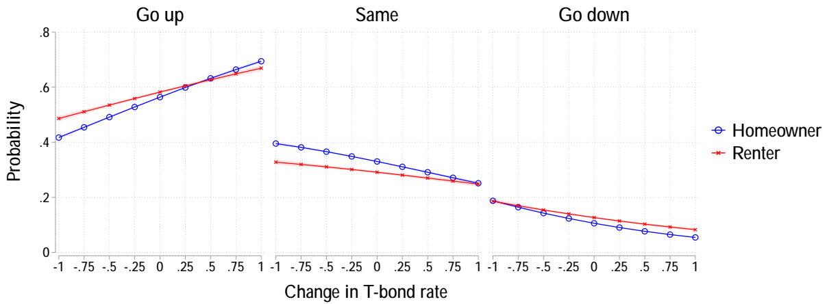
Figure 2: MARGINAL PROBABILITY OF HOUSEHOLD EXPECTATIONS OF INTEREST RATES
